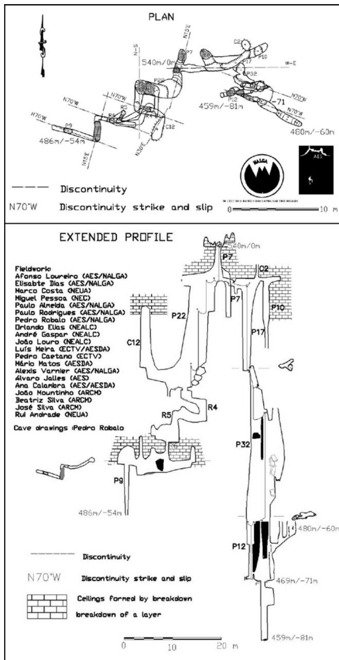
Fig. 3. Alecrineiros Shaft topography with geological survey.
